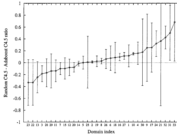
Figure 2. Difference in performance of Randomized C4.5 and Adaboosted C4.5. The difference is scaled by the error rate of C4.5 alone. Error bars give a 95% confidence interval according to the cross-validated t test (which tends to give intervals that are too narrow). The domains are numbered to correspond with the entries in Table 1.
